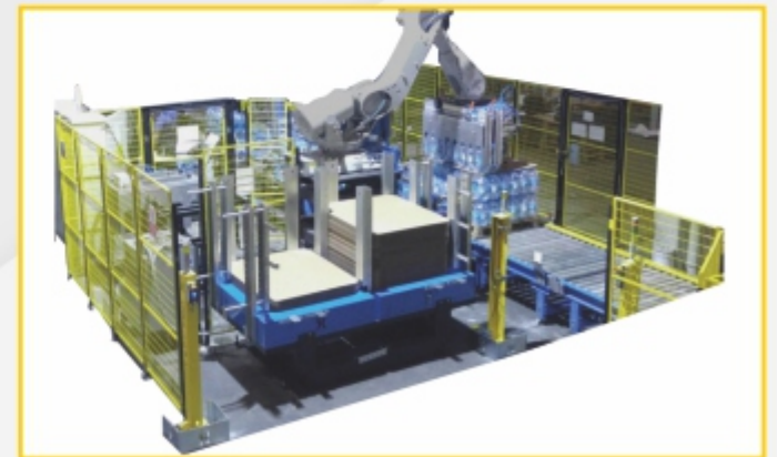
Shrink Bundled Products Robotic Palletizing
