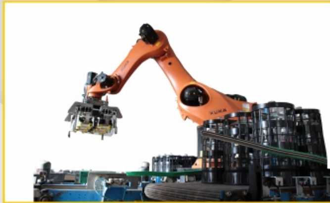
4 Gallon Glass with Baskets Robotic Palletizing Palletizing & De-Palletizing
